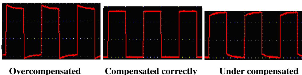
Figure 3-7 Displayed Waveforms of the Probe Compensation
