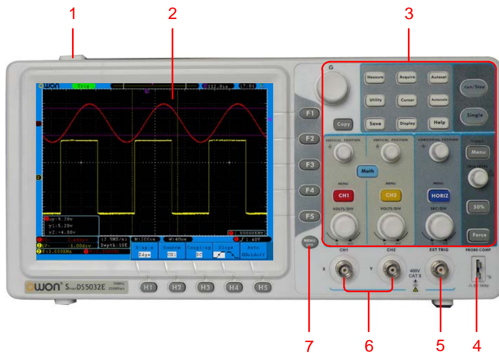
Figure 3-1 Front panel
